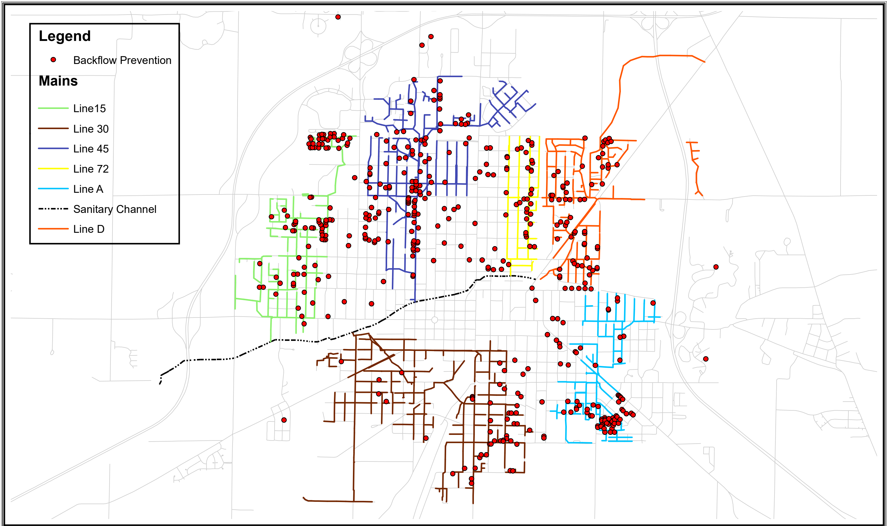
Backflow Prevention Locations
